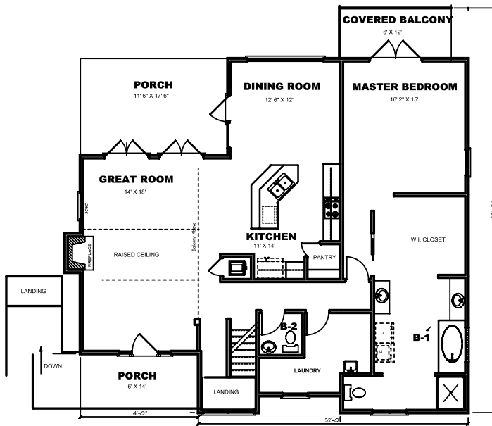
1 st FLOOR PLAN 1570 sf
